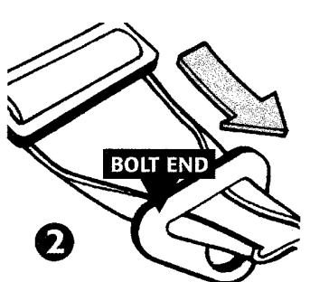
2 Fold both edges of webbing to center in order to pass through bolt end.
